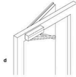
Overhead Installation(Frame Installation) On the other side of the door hinge
